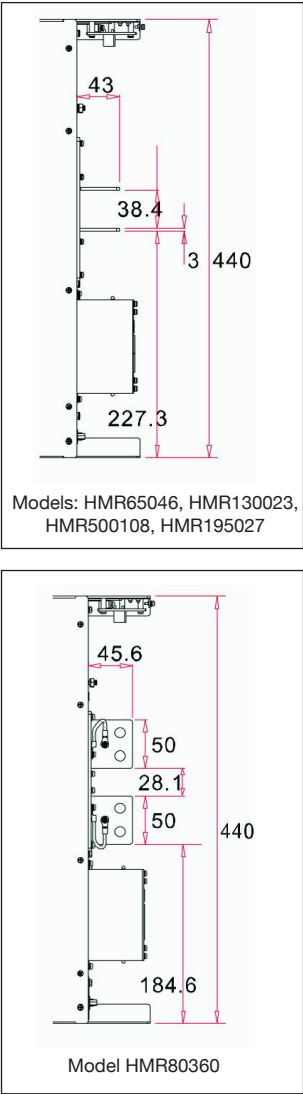
Output terminal measurements
