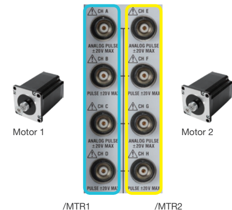
A single WT5000 configured for simultaneous, synchronized measurements from two motors to determine torque, rotation speed, direction, and electrical angles of A/B and Z phases.
