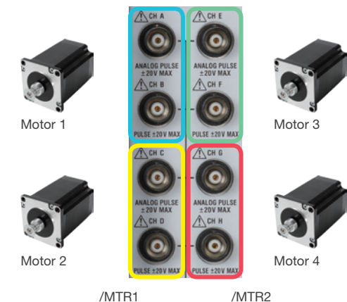
A single WT5000 configured for simultaneous synchronized measurements from four torque and rotation sensors to determine overall efficiency of four motors.
